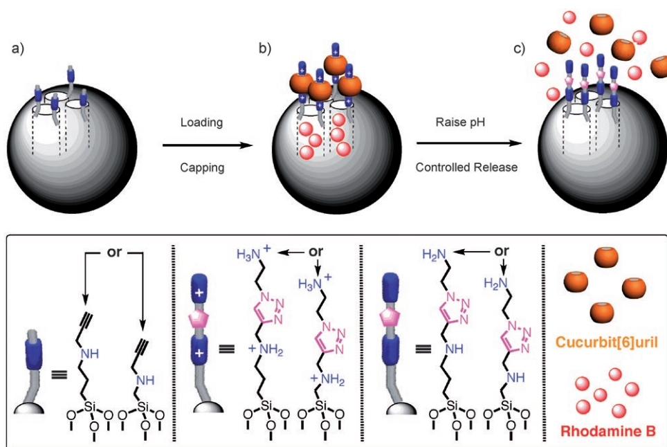
Figure 1. Graphical representations of operating supramolecular nanovalves \{3\text{C}\text{CB}[6]\} and \{6\text{C}\text{CB}[6]\} . The alkyne-functionalized mesoporous silica nanoparticles MCM-41 are loaded (a \rightarrow b) with rhodamine B (RhB) molecules, and capped (a \rightarrow b) with CB[6] during the CB[6]-catalyzed alkyne-azide 1,3-dipolar cycloadditions, followed by washing away the excess of substrates. RhB molecules are released (b \rightarrow c) by switching off the ion–dipole interactions between the CB[6] rings and the bisammonium stalks upon raising the pH value.
